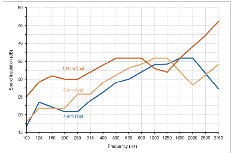
Figure 3 Acoustic Performance of Float Glass Source: Australian Fenestration Training Institute
