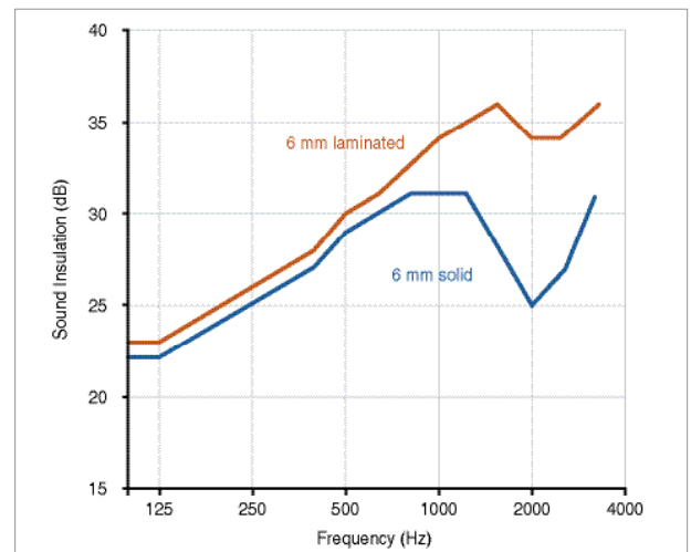
Figure 4 Acoustic Performance Comparison: Laminated Glass versus Float Glass. Source: Australian Fenestration Training Institute
