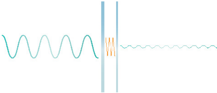
Figure 5 Sound waves as they propagate through laminated glass constructed with an acoustic interlayer. Source: Australian Fenestration Training Institute.
